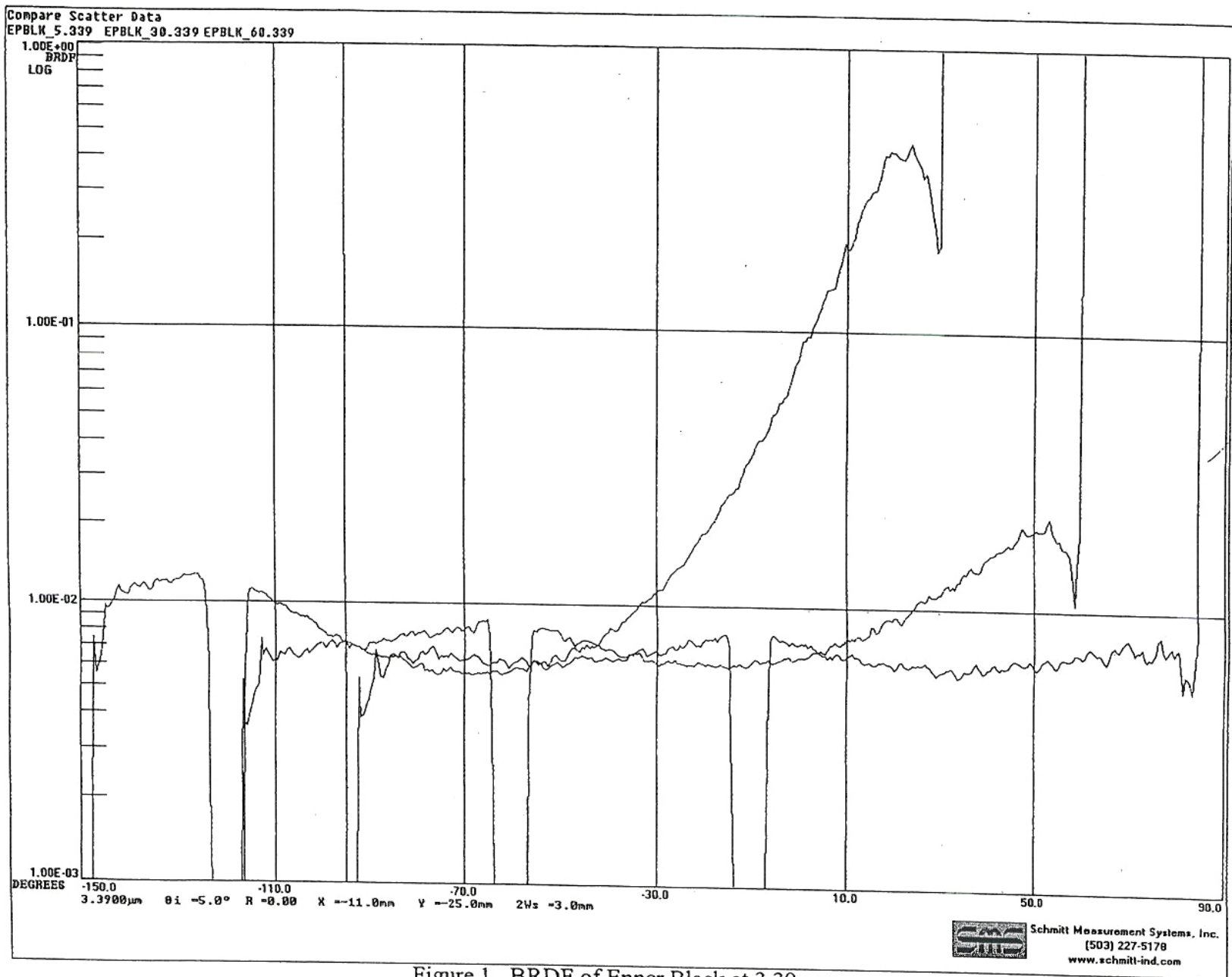
Figure 1. BRDF of Epner Black at 3.39 um
